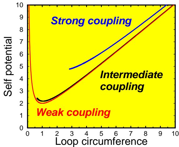
Figure 1.10: Variations of the self potential \Upsilon with the ring's circumference \ell = 2\pi r and the electromagnetic self coupling ( \lambda q^2 in the text). The red curve stands for various values of \lambda q^2 < 0.1 for which they are indistinguishable, and in the “safe” zone vorton-forming case; the minimum value of \Upsilon is then M , the vorton mass. \Upsilon for \lambda q^2 = 1 is represented as the black line, where it is clear that we now are in a zone where the potential has a minimum (new value for M ) but now terminates at some point. Finally the blue curve represents the potential for \lambda q^2 = 10 , an unrealistically large value, and this time the curve terminates even before reaching a minimum: this is a situation in which all loops with such parameters will eventually decay [Gangui, Peter & Boehm, 1998].
