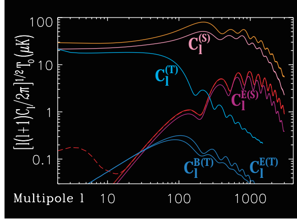
Figure 1.17: CMB Polarization for two different models. Red and orange (unlabeled) curves are the angular spectra derived for a \Lambda CHDM model, both with (red dashed line) and without (red full line) reionization. The temperature anisotropy spectrum from scalar perturbations (proportional to [C_\ell]^{1/2} , orange curve) is virtually unchanged for both ionization histories. The polarization spectrum ( \propto [C_\ell^{E(S)}]^{1/2} , red curves), although indistinguishable for \ell \gtrsim 20 , dramatically changes for small \ell 's; in this model the Universe is reionized suddenly at low redshift with optical depth \tau_c = 0.05 . Blue and violet curves represent a SCDM model but with a high tensor-mode amplitude, T/S=1 at the quadrupole ( \ell = 2 ) level, with scale-invariant spectral indices n_s = 1 and n_T = 0 . Separate scalar (noted C_\ell^{(S)} ) and tensor ( C_\ell^{(T)} ) contributions to temperature anisotropies are shown (top curves). Scalar modes only generate E-type polarization ( C_\ell^{E(S)} ), which is smaller than the corresponding red curve of the \Lambda CHDM model both due to differences in the models (notably \Lambda \neq 0 for the red curves) and due to the influence of tensors on the normalization at small \ell . E- and B-type polarization from tensor modes are also shown, respectively C_\ell^{E(T)} and C_\ell^{B(T)} . Model spectra were computed with CMBFAST and are normalized to \delta T_{\ell=10} = 27.9 \mu\text{K} .
