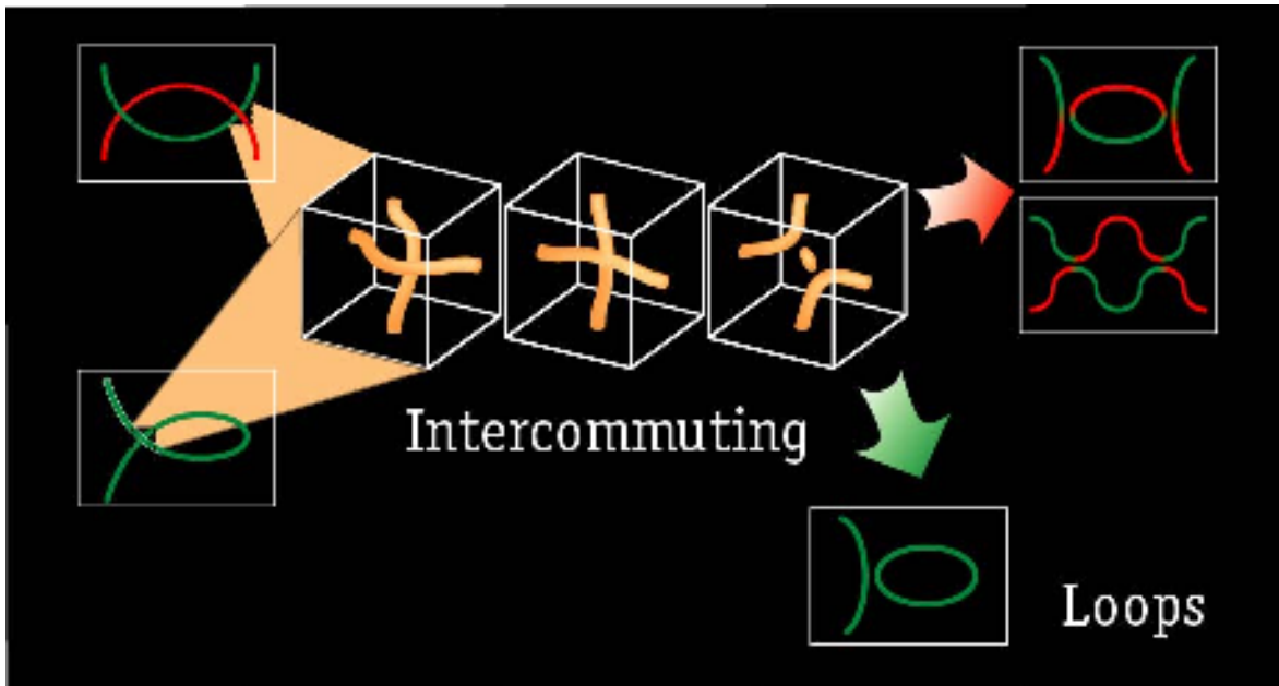
Figure 1.5: Global string interactions leading to loop formation. Whenever two string segments intersect, they reconnect or intercommute (green and red strings – upper part of the figure). Analogously, if a string intersects itself, it can break off a closed loop (green string – bottom part of the figure). In both cases, the interacting string segments first suffer a slight deformation (due to the long-range forces present for global strings), they subsequently fuse and finally exchange partners. A ephemeral unstable amount of energy in the form of a small loop remains in the middle where the energy is high enough to place the Higgs field in the false vacuum. It then quickly collapses, radiating away its energy. The situation is roughly the same for local strings, as simulations have shown.
