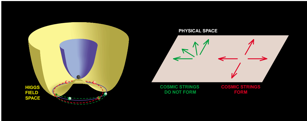
Figure 1.3: The complex scalar Higgs field evolves in a temperature-dependent potential V(\phi) . At high temperatures (violet surface) the vacuum expectation value of the field lies at the bottom of V . For lower temperatures, the potential adopts the “Mexican hat” form (yellow surface) and the field spontaneously chooses one amongst the new available (degenerate) lowest energy states (the violet circle along the valley of the hat). This isolates a single value/direction for the phase of the field, spontaneously breaking the symmetry possessed by the system at high energies. Different regions of the universe, with no causal connection, will end up having arbitrarily different directions for the field (arrows on the right). As separate regions of broken symmetry merge, it is not always possible for the field orientations to match. It may happen that a closed loop in physical space intersects regions where the Higgs phase varies from 0 to 2\pi (red arrows, corresponding to the red dashed-line on the left panel). In that situation, a cosmic string will pass somewhere inside the loop. On the contrary, green arrows (and green dashed-line on the left panel) show a situation where no string is formed after the phase transition.
