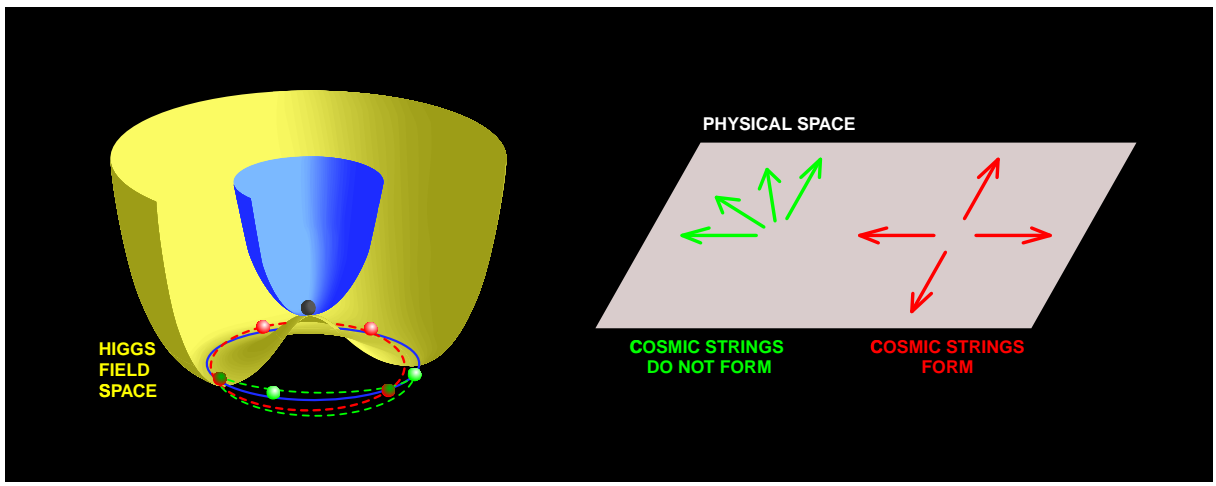
FIG. 3: The complex scalar Higgs field evolves in a temperature-dependent potential V(\phi) . At high temperatures (violet narrow surface) the vacuum expectation value of the field lies at the bottom of V . For lower temperatures, the potential adopts the “Mexican hat” form (yellow surface) and the field spontaneously chooses one amongst the new available (degenerate) lowest energy states (the violet circle along the valley of the hat). This isolates a single value/direction for the phase of the field, spontaneously breaking the symmetry possessed by the system at high energies. Different regions of the universe, with no causal connection, will end up having arbitrarily different directions for the field (arrows on the right). As separate regions of broken symmetry merge, it is not always possible for the field orientations to match. It may happen that a closed loop in physical space intersects regions where the Higgs phase varies from 0 to 2\pi (red arrows, corresponding to the red dashed-line on the left panel). In that situation, a cosmic string will pass somewhere inside the loop. On the contrary, green arrows (and green dashed-line on the left panel) show a situation where no string is formed after the phase transition.
