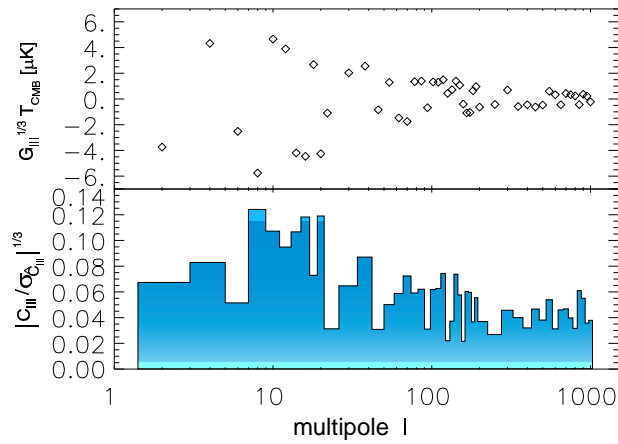
FIG. 12: The CMB angular bispectrum in the ‘diagonal’ case ( G_{ll}^{1/3} ) from wiggly cosmic strings in a spatially flat model with cosmological parameters \Omega_{\text{CDM}} = 0.3 , \Omega_{\text{baryon}} = 0.05 , \Omega_{\Lambda} = 0.65 , and Hubble constant H = 0.65 \text{ km s}^{-1} \text{ Mpc}^{-1} [upper panel]. In the lower panel we show the ratio of the signal to theoretical noise |C_{ll}/\sigma_{C_{ll}}|^{1/3} for different multipole indices. Normalization follows from fitting the power spectrum to the BOOMERANG and MAXIMA data.
