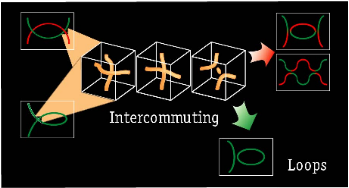
FIG. 5: Global string interactions leading to loop formation. Whenever two string segments intersect, they reconnect or intercommute (green and red strings – upper part of the figure). Analogously, if a string intersects itself, it can break off a closed loop (green string – bottom part of the figure). In both cases, the interacting string segments first suffer a slight deformation (due to the long-range forces present for global strings), they subsequently fuse and finally exchange partners. A ephemeral unstable amount of energy in the form of a small loop remains in the middle where the energy is high enough to place the Higgs field in the false vacuum. It then quickly collapses, radiating away its energy. The situation is roughly the same for local strings, as simulations have shown.
